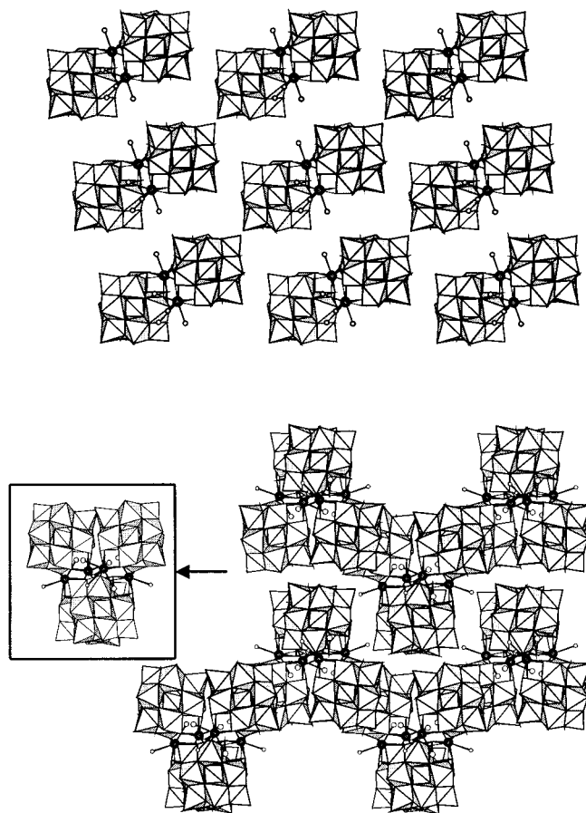
Figure 3. Packing of anions in planes perpendicular to chain axis. Top: 1 viewed down the crystallographic a axis. Bottom: 2 viewed down the crystallographic c axis. The a axis is horizontal. The inset shows a view down a single anion chain of 2 .
